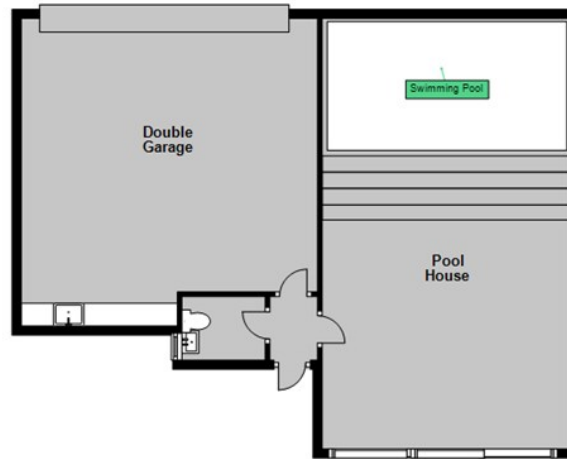
Ground Floor Approx. 146.6 sq. metres (1578.0 sq. feet)
